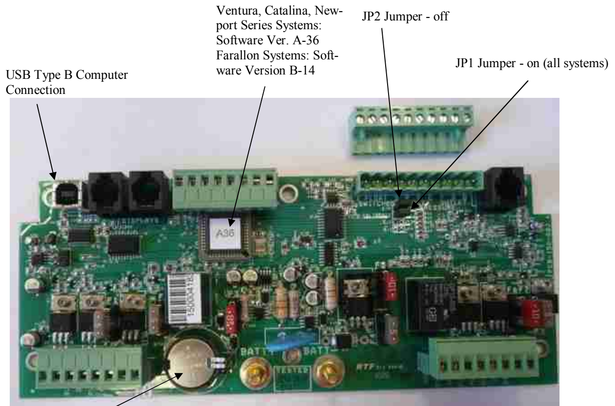
Spectra MPC-5000 CONTROLS printed circuit
